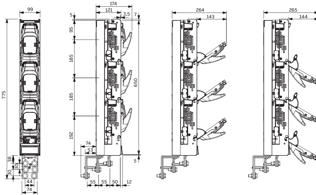
BZL1250A-1P-M12
