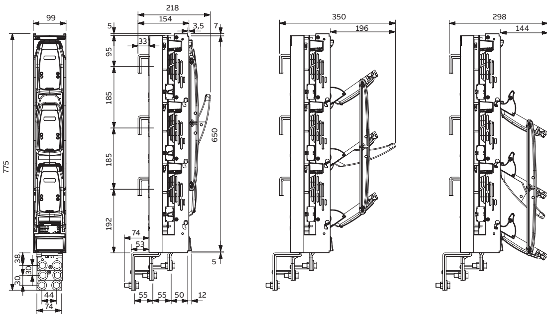
BZH1250A-3P-M12
