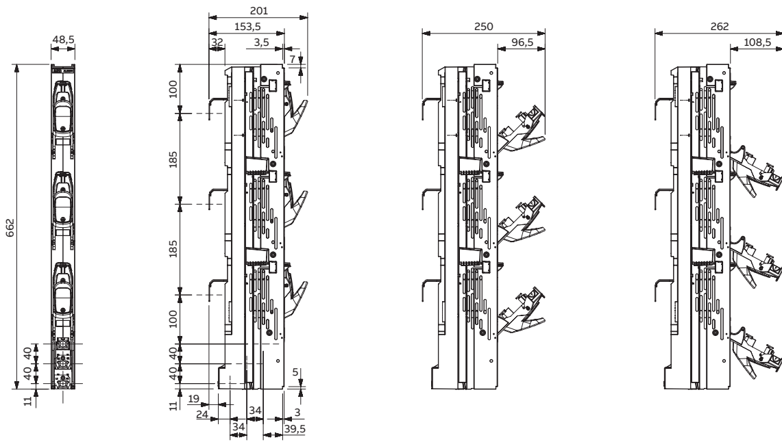
ZHBM00-1P
