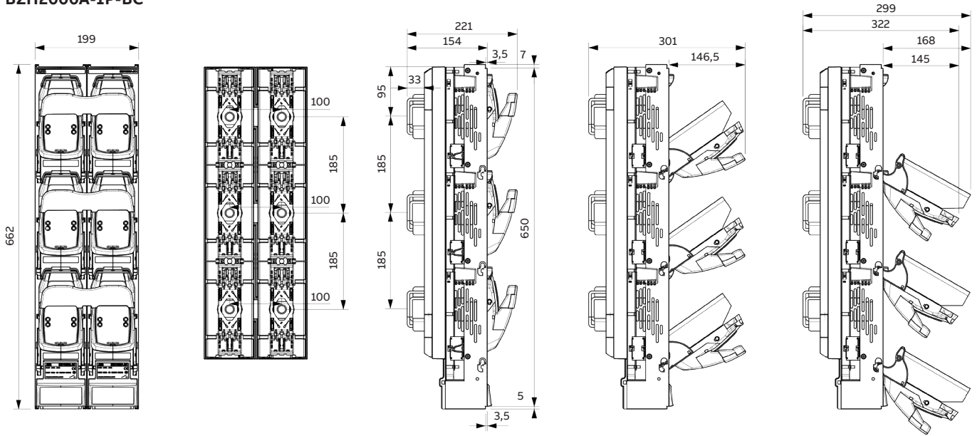
BZH2000A-1P-BC
